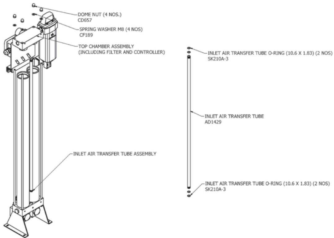
Figure 18. Exploded view of Dryspell Plus models 20 and 30
