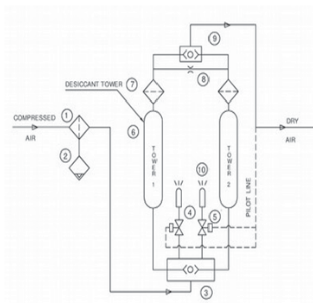
Figure 3. Schematic of Dryspell Plus dryer
