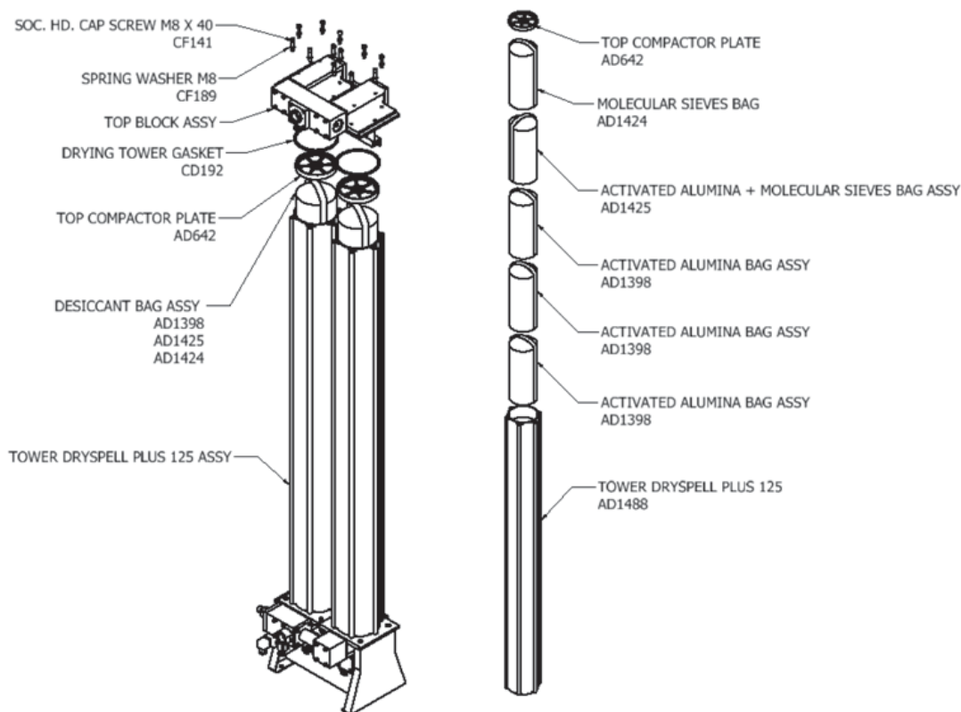
Figure 26. Changing desiccant-Dryspell Plus model 125
