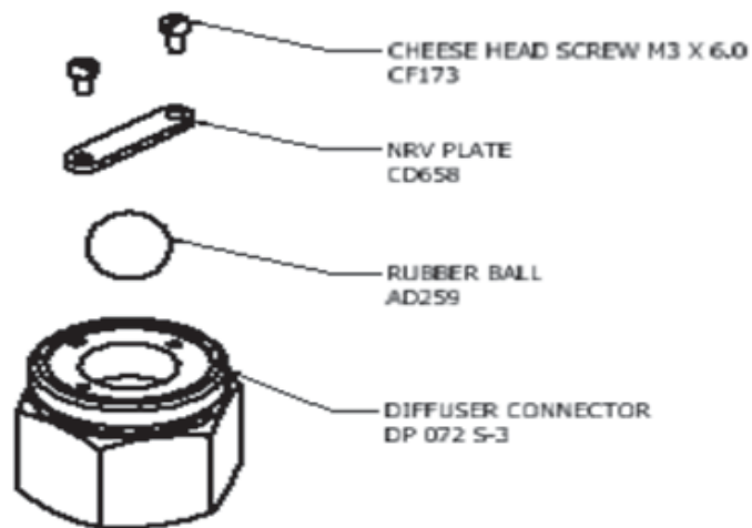
Figure 12. Exploded view of non-return valve
