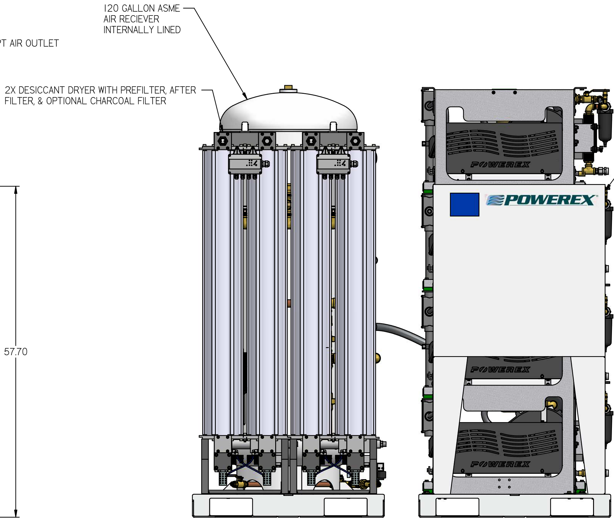
FRONT VIEW
