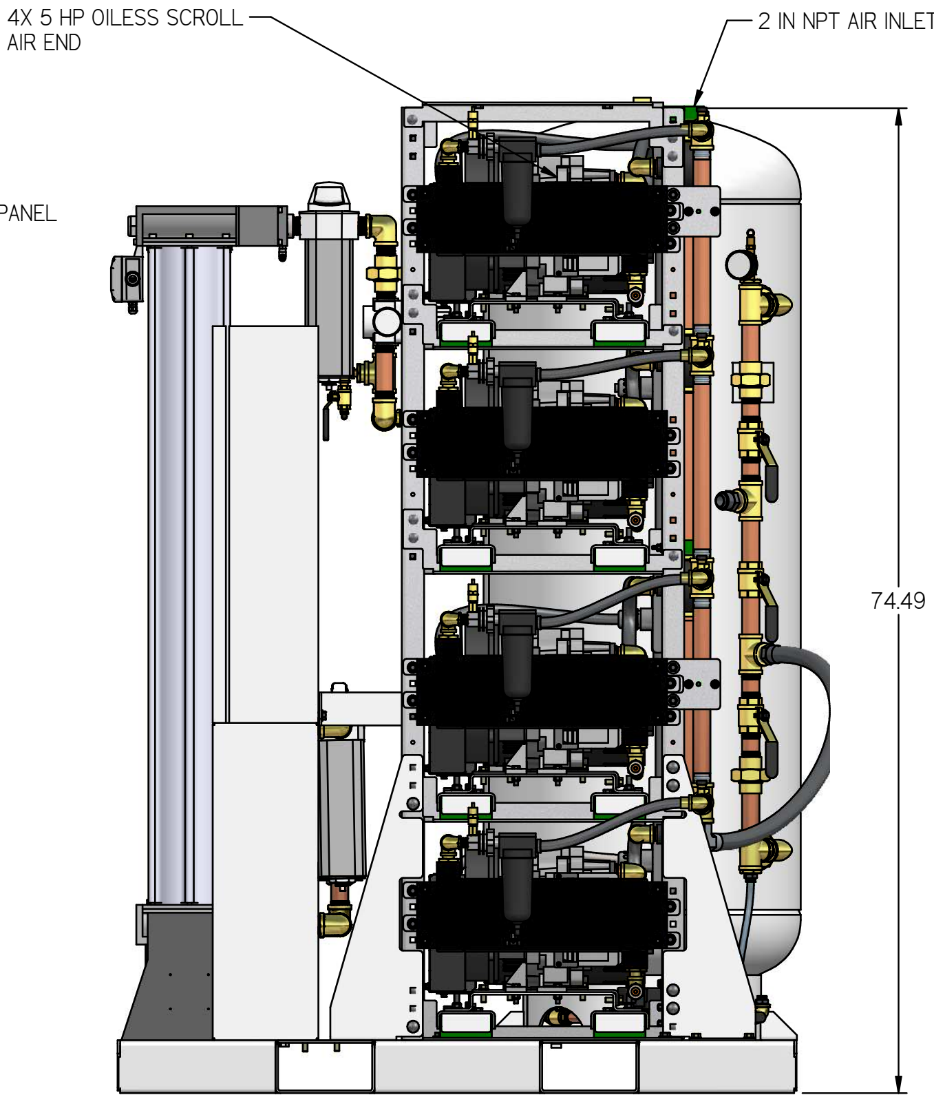
LEFT VIEW
