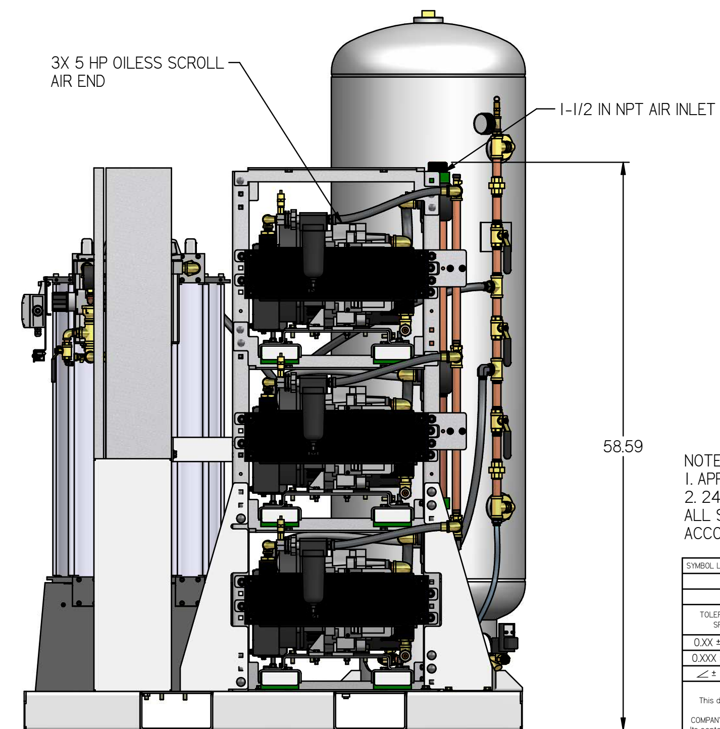
LEFT VIEW
