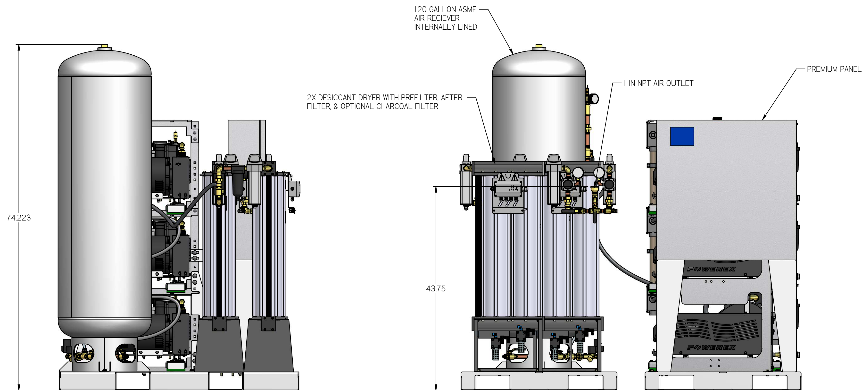
FRONT VIEW
